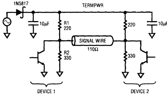
Figure 2. Passive Termination
